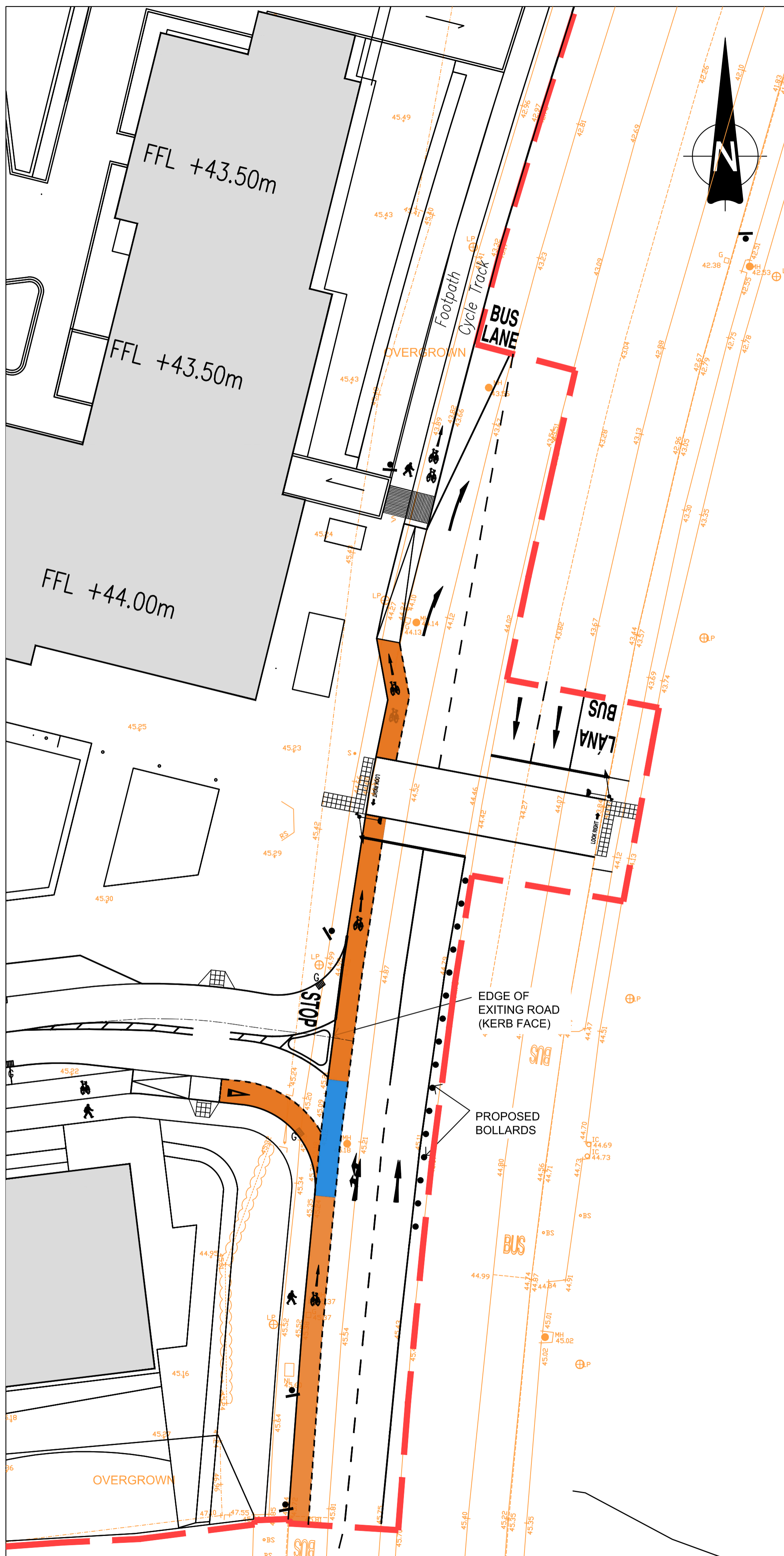
PLAN VIEW – PROPOSED LEFT IN LEFT OUT JUNCTION SCALE 1:250
