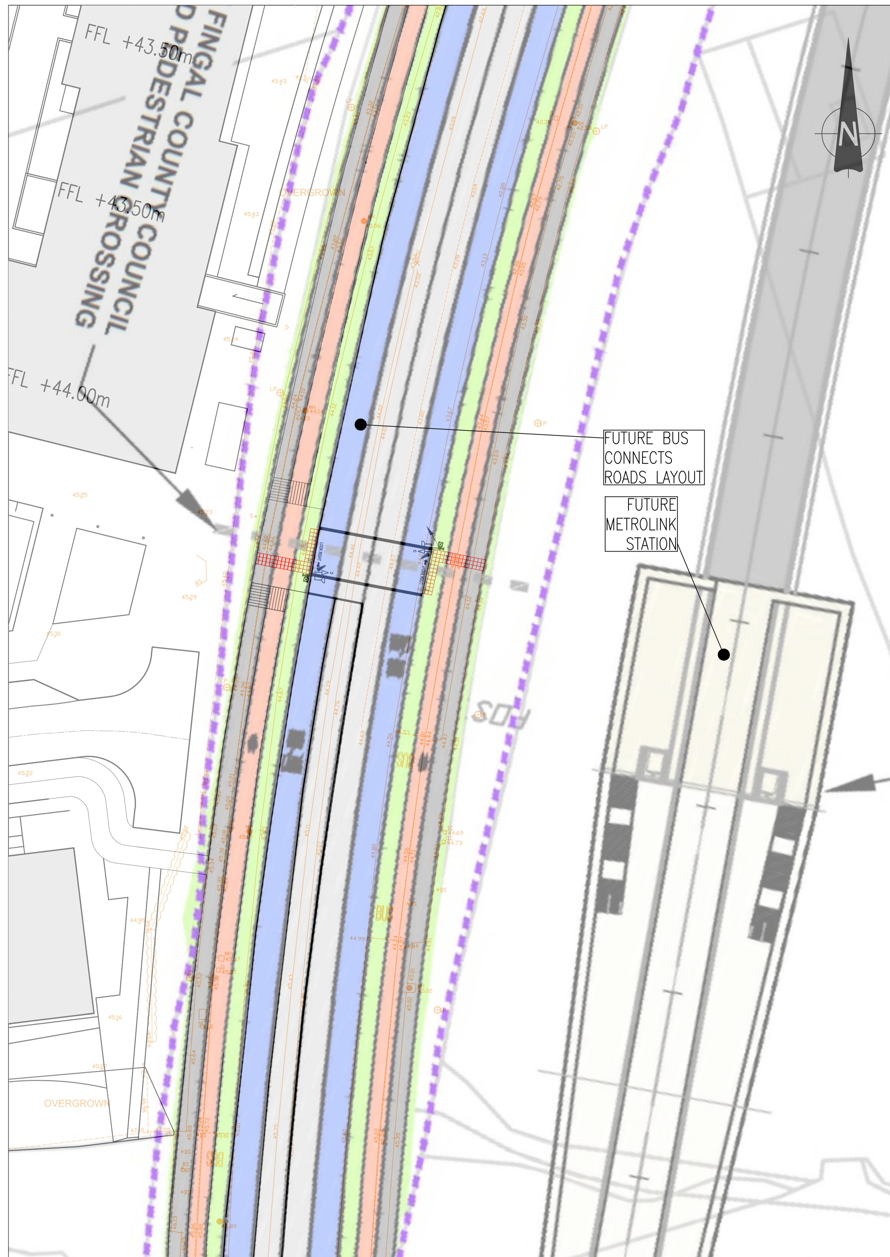
PLAN VIEW – FUTURE RESIDENTIAL CUL DE SAC. (FUTURE BUS CONNECTS ROADS LAYOUT & METROLINK STATION) SCALE 1:250
